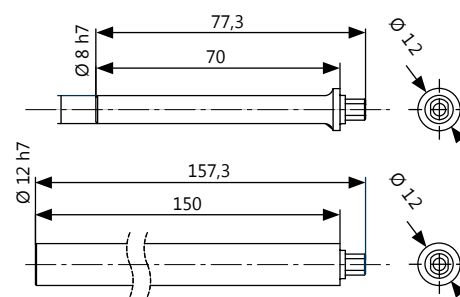
Sketch 2 Type M (short)
